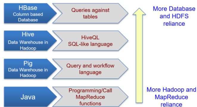
Figure 3. Query languages for Hadoop
