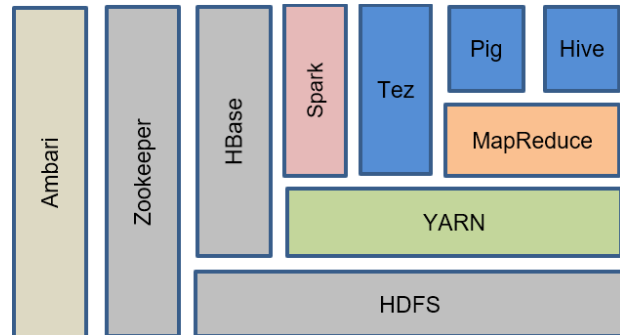
Figure 2. Main components of the Hadoop ecosystem
