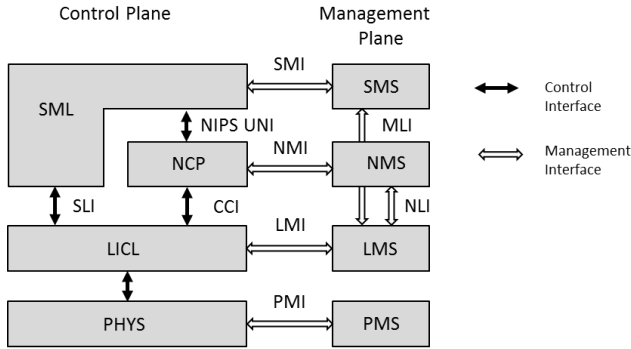
Figure 7. GEYSERS control and management architecture and interfaces.
